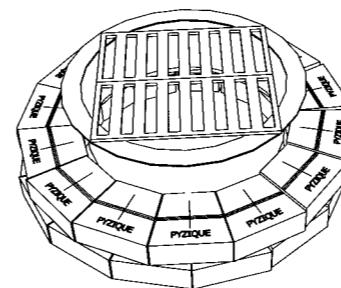
Figure 2. Layer 2 / Wallstone placement.
