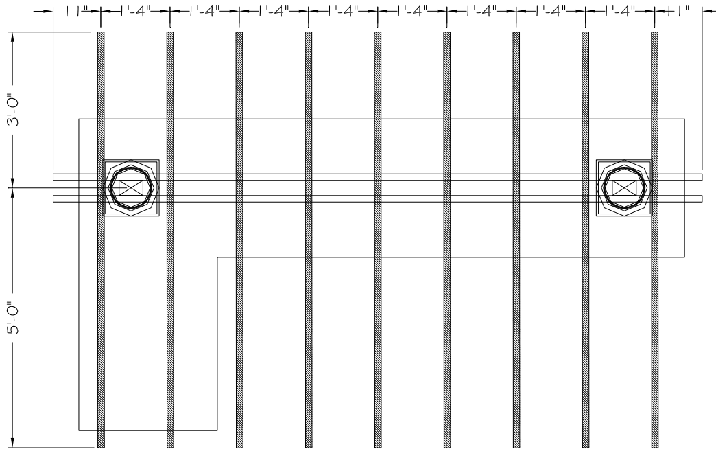
ROOF PLAN
