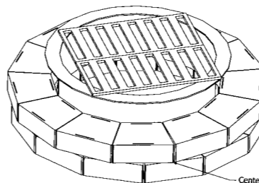
Figure 2. Layer 2 / Wallstone placement.
