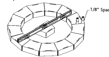
Figure 1. Layer 1 / Wallstone placement.
