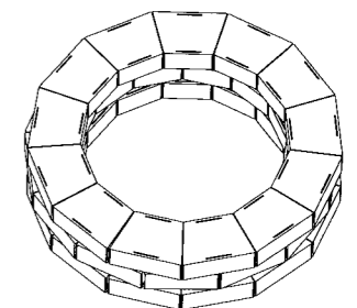
Figure 3. Layer 3 / Wallstone placement.
