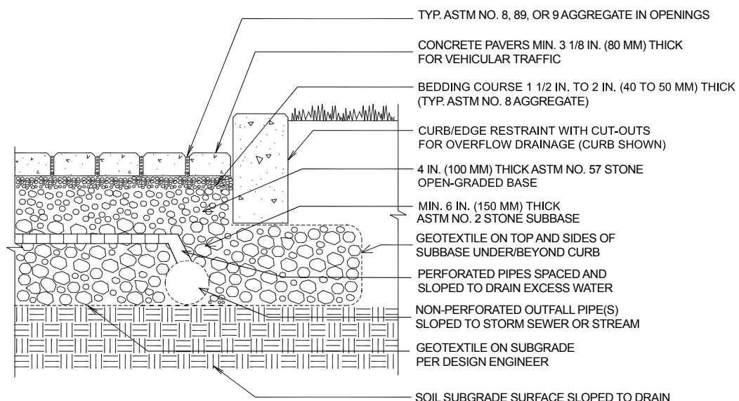
Figure 6. Partial exfiltration through the soil subgrade. Perforated pipes can be raised above the soil subgrade to drain water from higher depth rainstorms. Smaller storms which often contain higher pollutant concentrations can be captured below the perforated pipes, stored and infiltrated.
