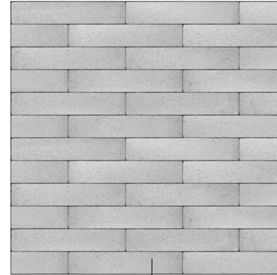
Wall Stone - Concrete - Cambridge Pavers - Olde English Non Tumbled Wall 4 x 8 x 20 - Running Bond - Platinum
