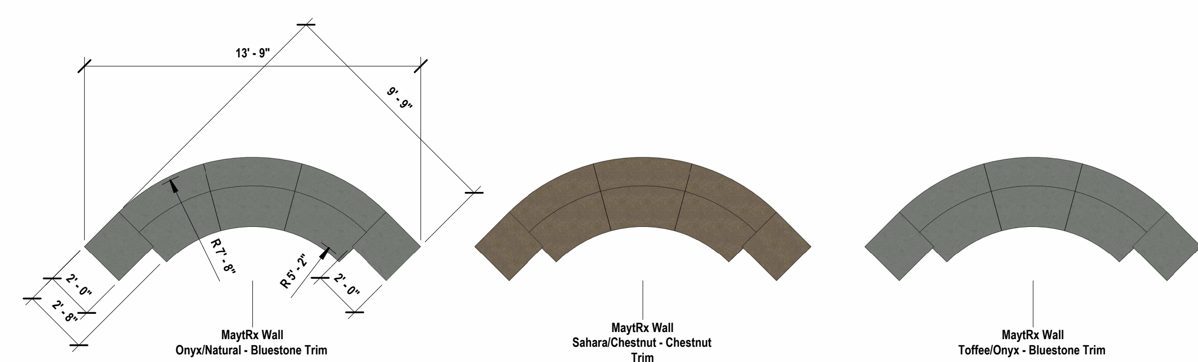
PRE-PACKAGED MAYTRX SEATING WALL KIT - QUARTER ROUND
