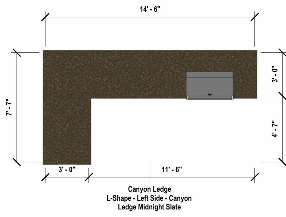
PLAN VIEW
