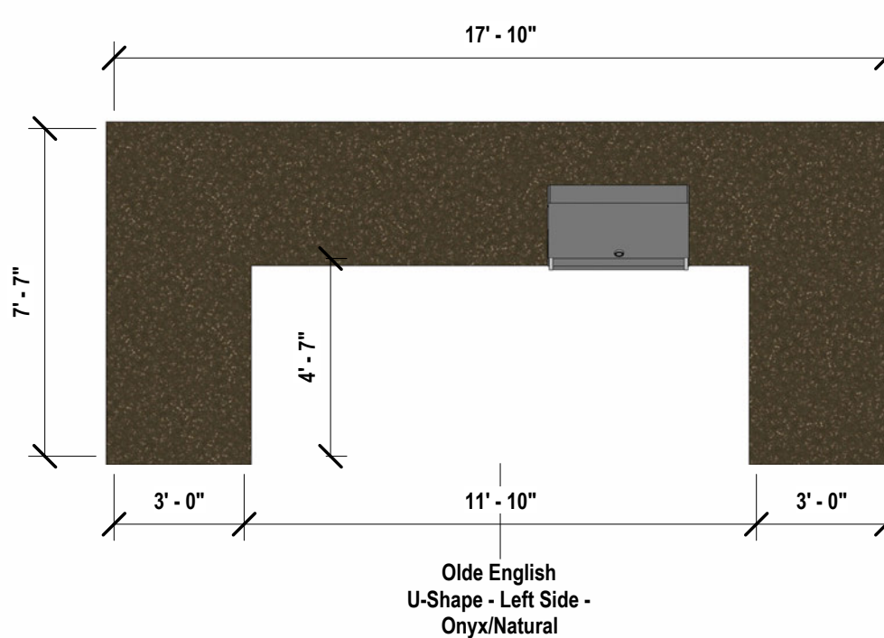
U SHAPED
